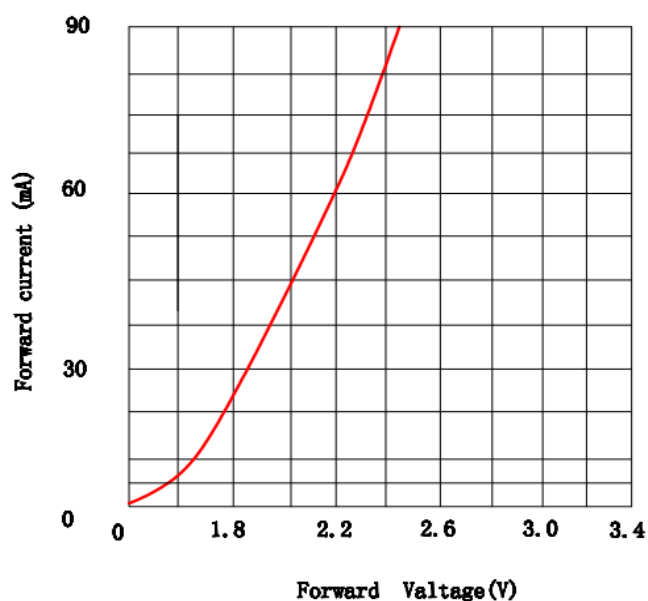
Forward Current VS. Forward Voltage 电压与电流关系曲线图
