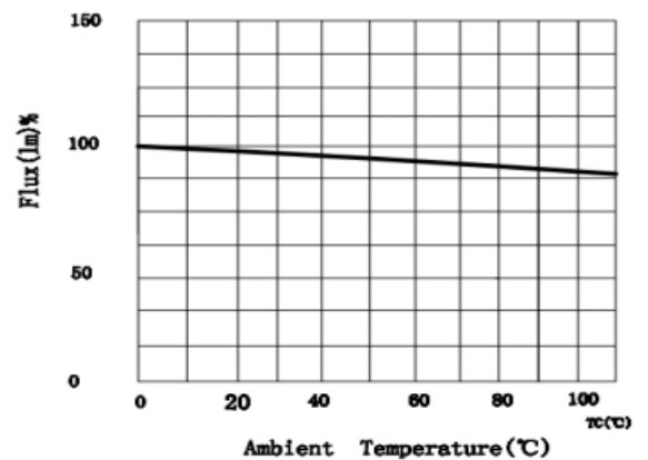
Relative Luminous Flux VS. Ambient Temperature 温度与亮度关系曲线图
