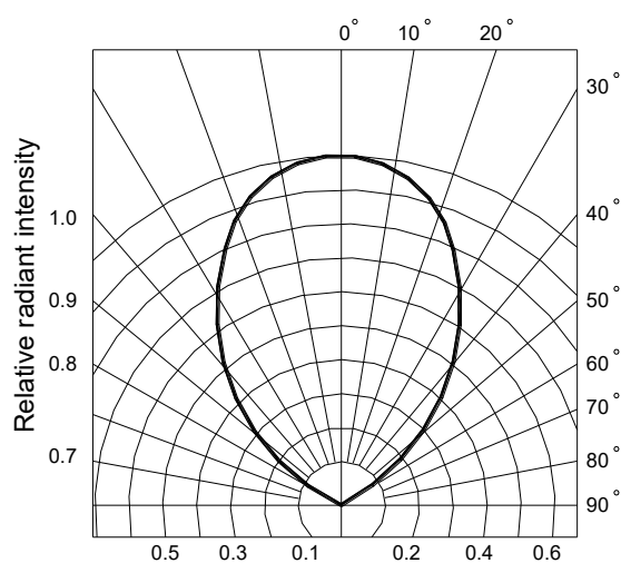
Fig.6 Radiation diagram
