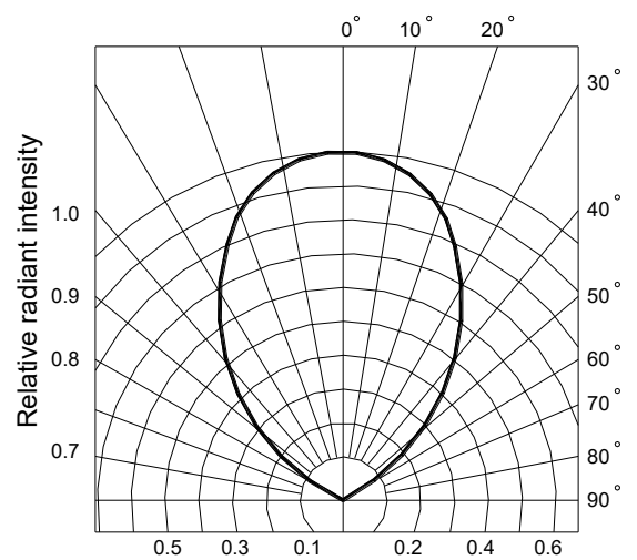
Fig.6 Radiation diagram
