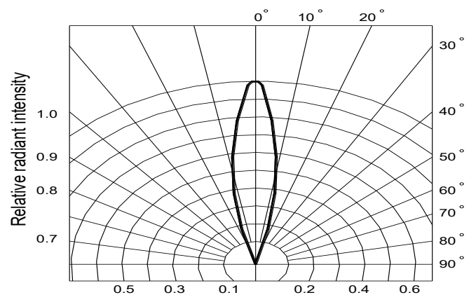
Fig.6 Radiation diagram
