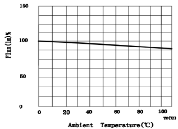
Relative Luminous Flux VS. Ambient Temperature 温度与亮度关系曲线图
